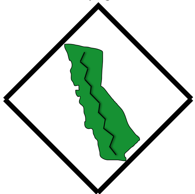
Earthquake Fault Line
